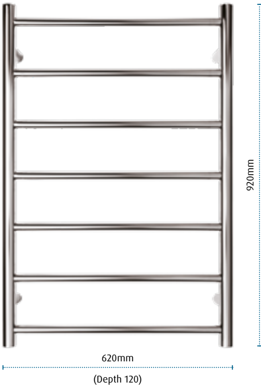
Commercial 7 bar ROUND HTR-TR0701M
