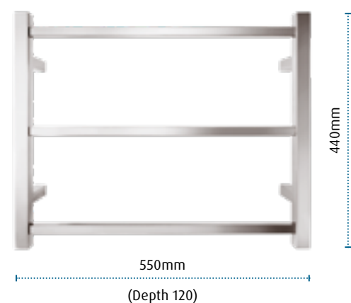
Retro Fit 3 bar SQUARE HTR-TS0304LP (LHS plug in only) Non-heated model also available TR-TS0304
