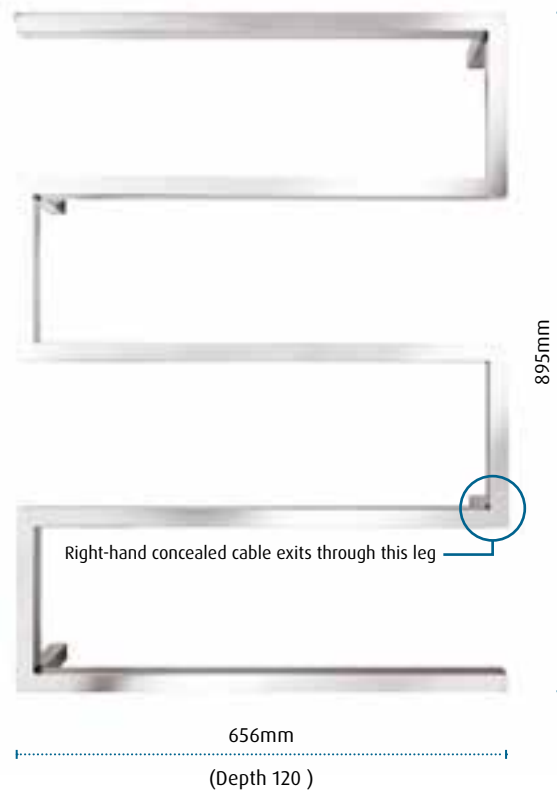
Designer Snake Rail SQUARE HTR-5HS9065
