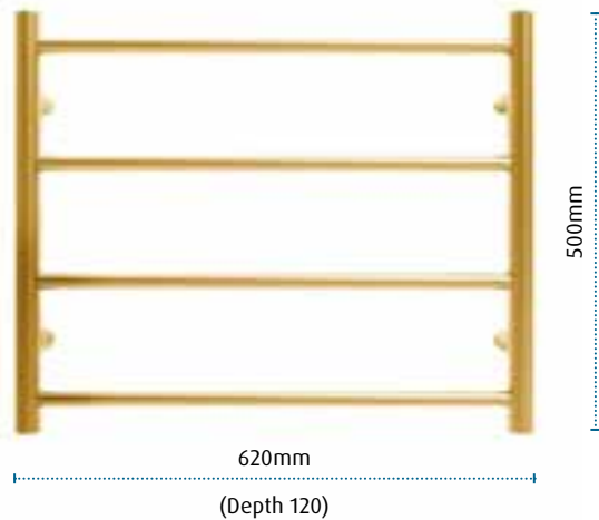
Commercial 4 bar ROUND – PVD BRUSHED GOLD HTR-TR0402MBG
