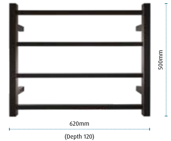
Black satin 4 bar SQUARE HTR-TS0402MBL
