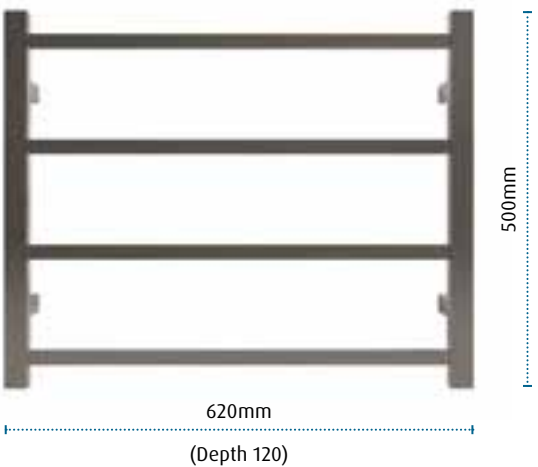
Commercial 4 bar SQUARE – PVD BRUSHED GUN METAL GREY HTR-TS0402MGR
